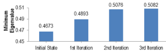
Figure 5 Eigenvalue at each iteration
