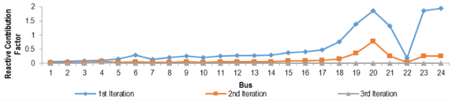
Figure 3 Reactive Contribution Factor (RCF) computation iteration process
