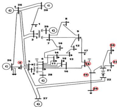
Figure 1 The IEEE 30-bus Reliability Test System (Saadat, 1999)
