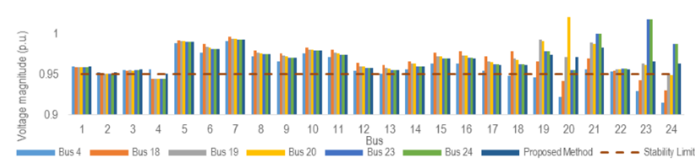
Figure 6 Comparison of voltage magnitude at different placement and proposed method
