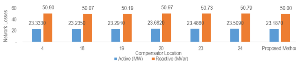
Figure 7 Comparison of network losses
