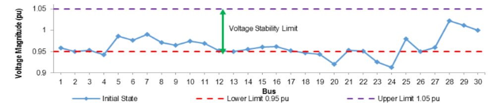
Figure 2 Voltage magnitude at the initial state
