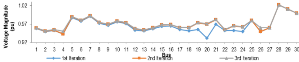
Figure 4 Voltage profile improvement at each iteration
